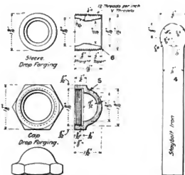
Figs. 286-291. Late Flexible Staybolt. Flannery Bolt Co.
